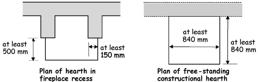
Figure 3.41 Hearth construction
