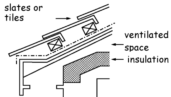
Figure 3.32 Roof type A insulation on a level ceiling
