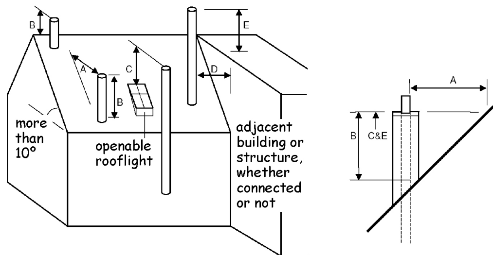
Figure 3.52 Solid fuel - flue outlets
