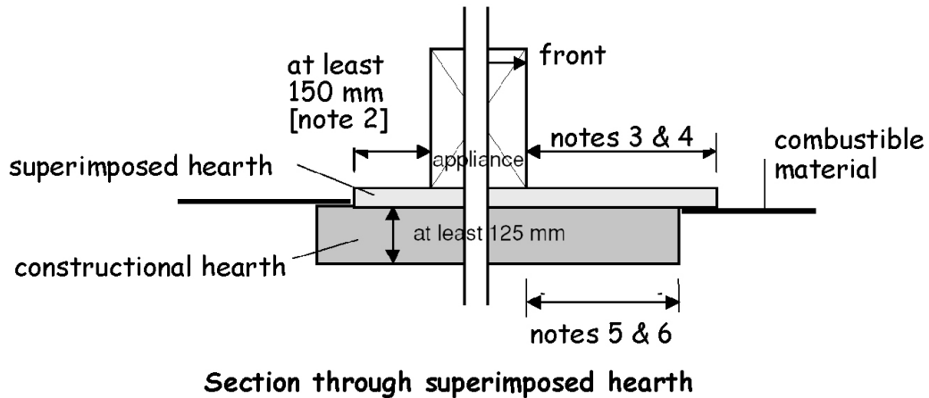
Figure 3.43 Superimposed hearths
