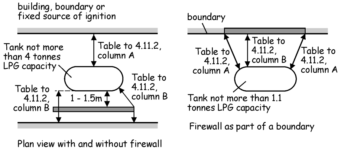
Figure 4.13 Separation or shielding of a LPG tank from a building, boundary or fixed source of ignition
