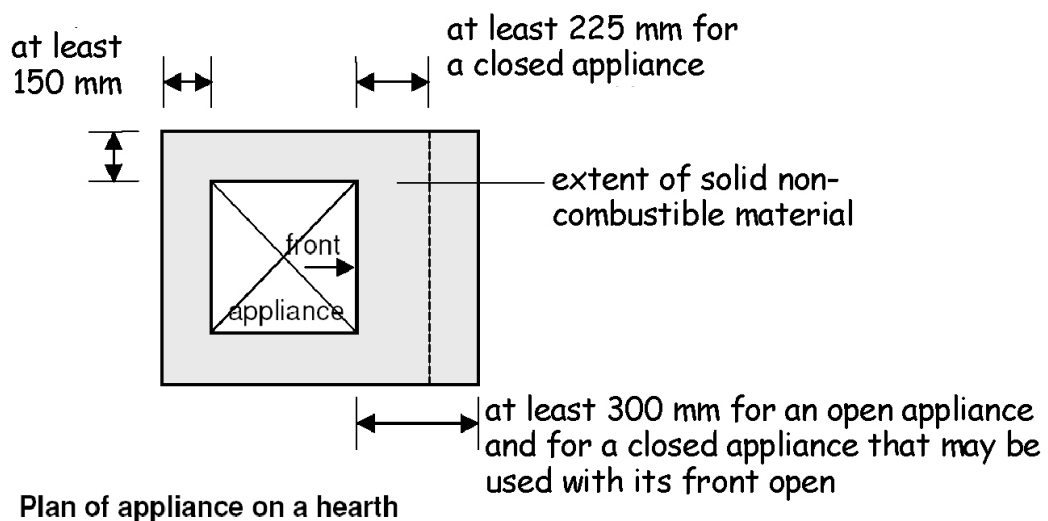
Figure 3.42 Appliance location
