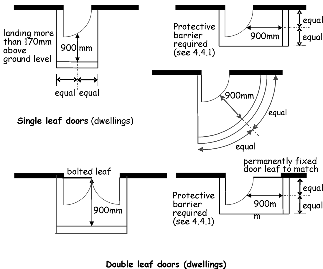
Figure 4.9 Landings serving outward-opening fully glazed doors
