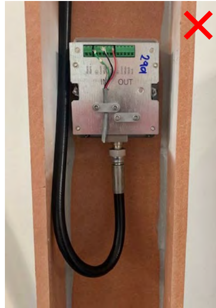
Figure 54: At risk trunking installation with hose bending
