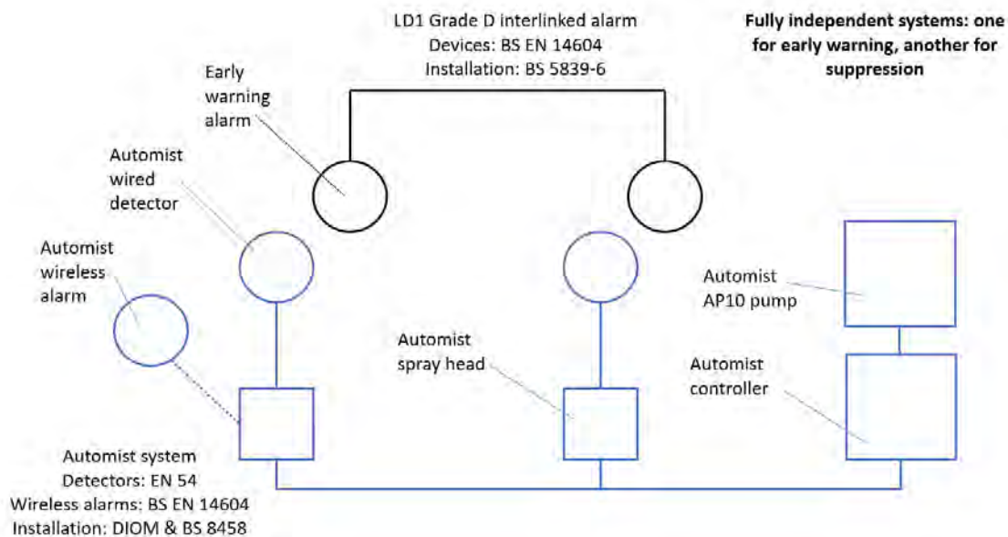
Figure 42: Early warning and suppression system independent systems
