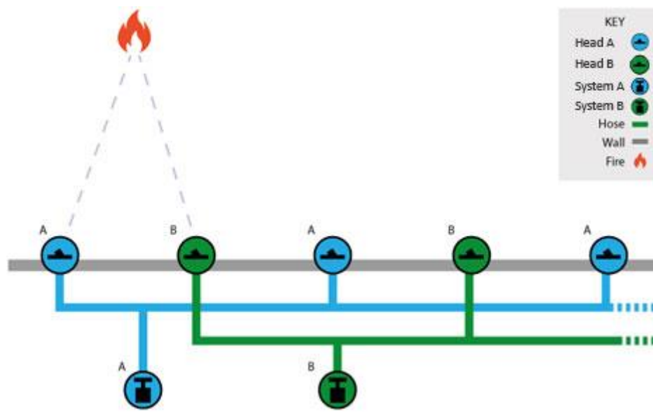
Figure 36: Installing two Automist systems in parallel
