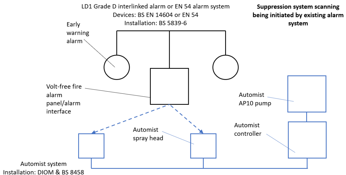
Figure 45: Volt-free fire panel or interface used to initiate scanning of Automist
