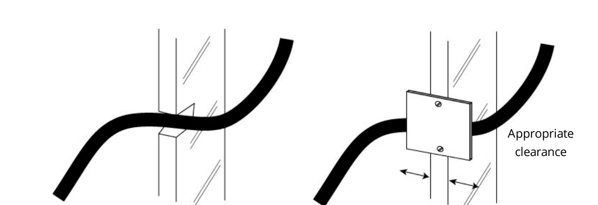
Figure 52: Example of mechanical protection within a joist
