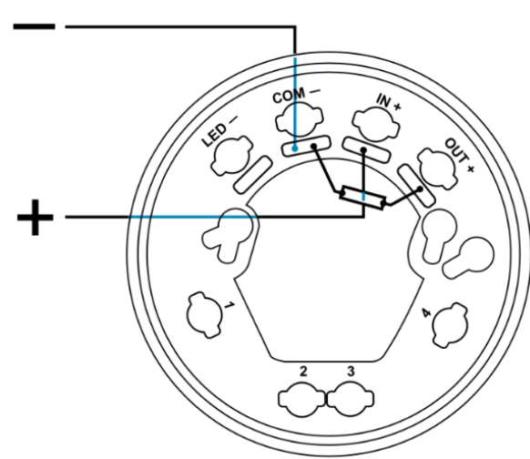
Figure 56: Mounting the resistor on wired Apollo detector
