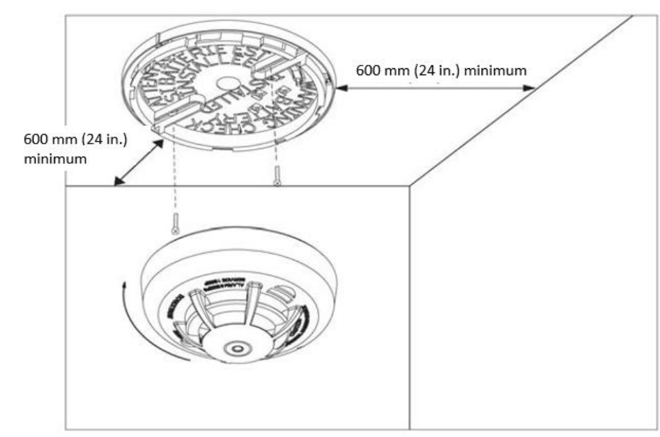
Figure 58: Mounting the detector
