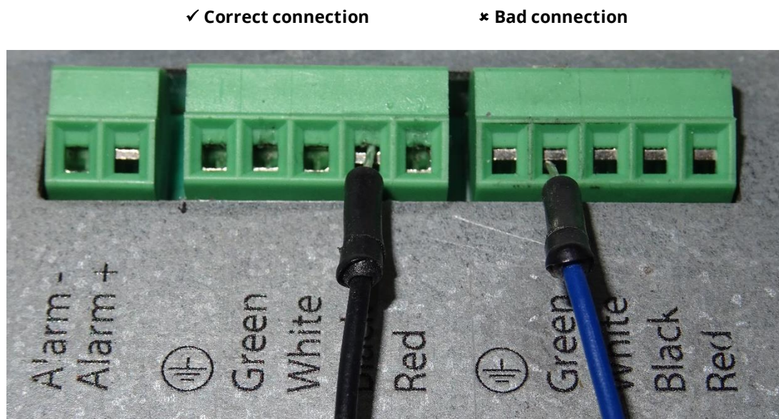
Figure 70: Connections on the spray head
