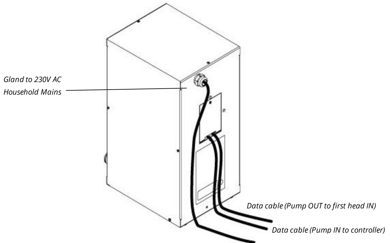
Figure 74: The pump front panel
