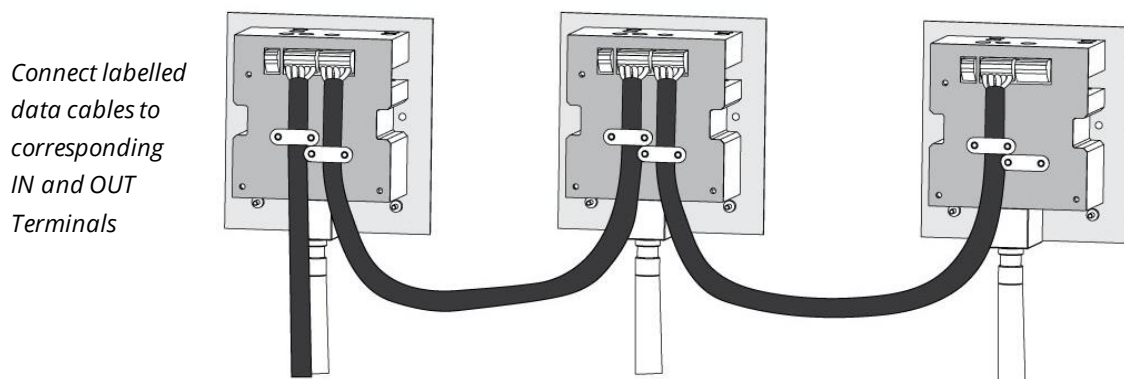
Figure 71: Spray head daisy chain connection
