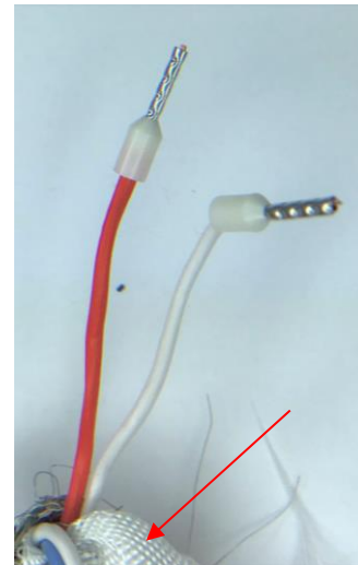
Figure 66: Alarm Cable with 0.5mm2 ferrule
