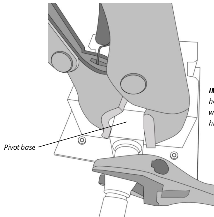
Figure 73: Spray head water path connection
