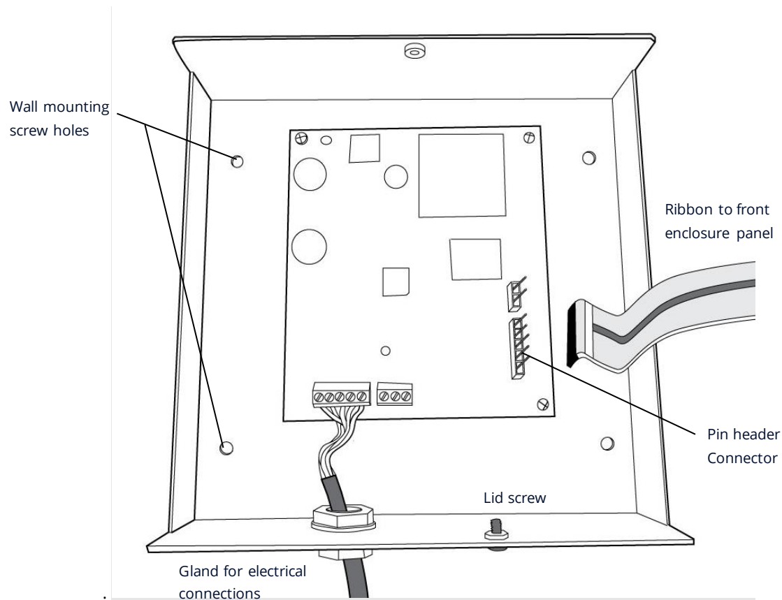
Figure 60: Connecting the controller
