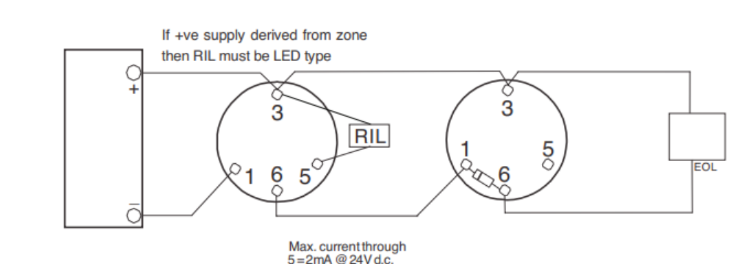
Figure 55: Wiring for Plumis DT02 wired detector
